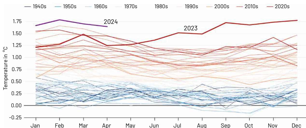
Figure 1: Monthly global average temperatures anomaly from the 1940s to 2024
